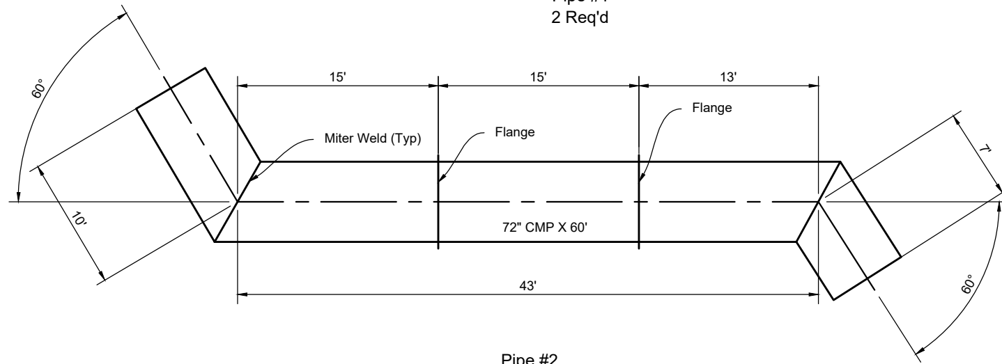
Pipe #2 2 Req'd
