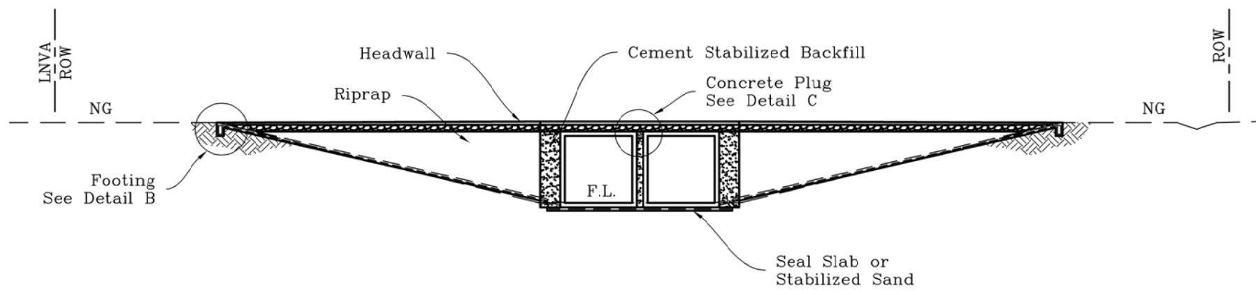
Rock Drive Crossing - (2) 10'X10'X22' Concrete Box Culverts STA 57+99
