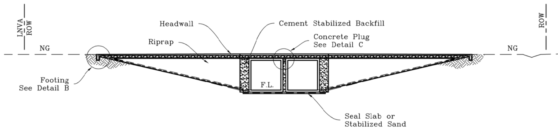
Rock Drive Crossing - (2) 10'X10'X22' Concrete Box Culverts STA 11+71
