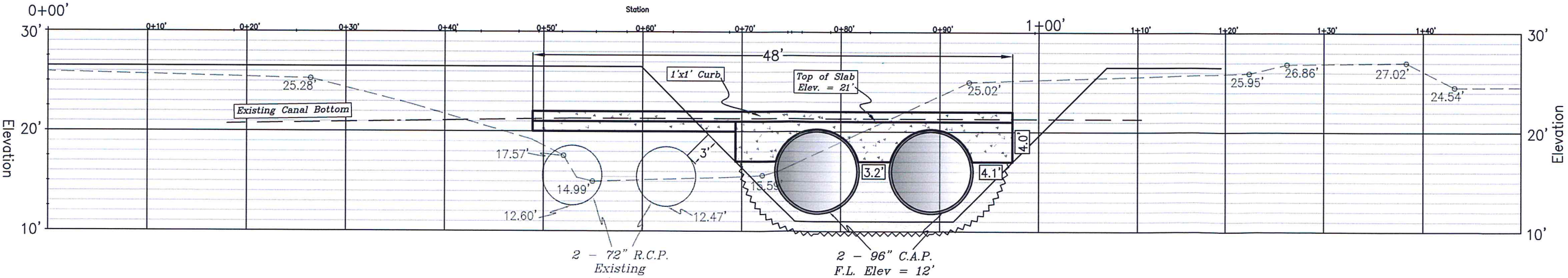
Profile of Ditch 608 on East side of canal
