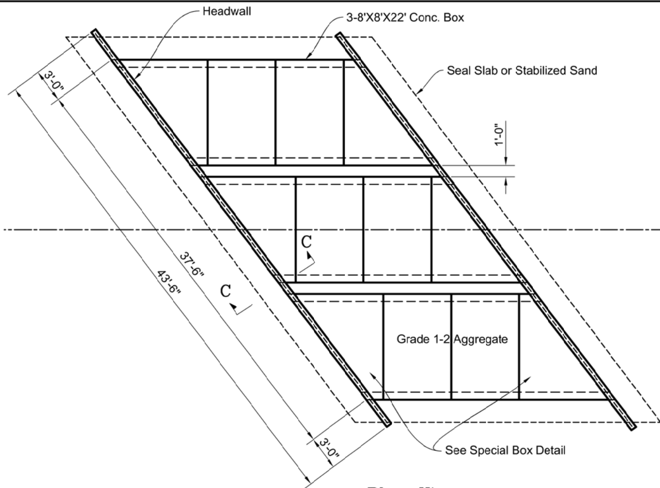
Plan View
