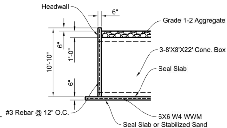
Section C-C
