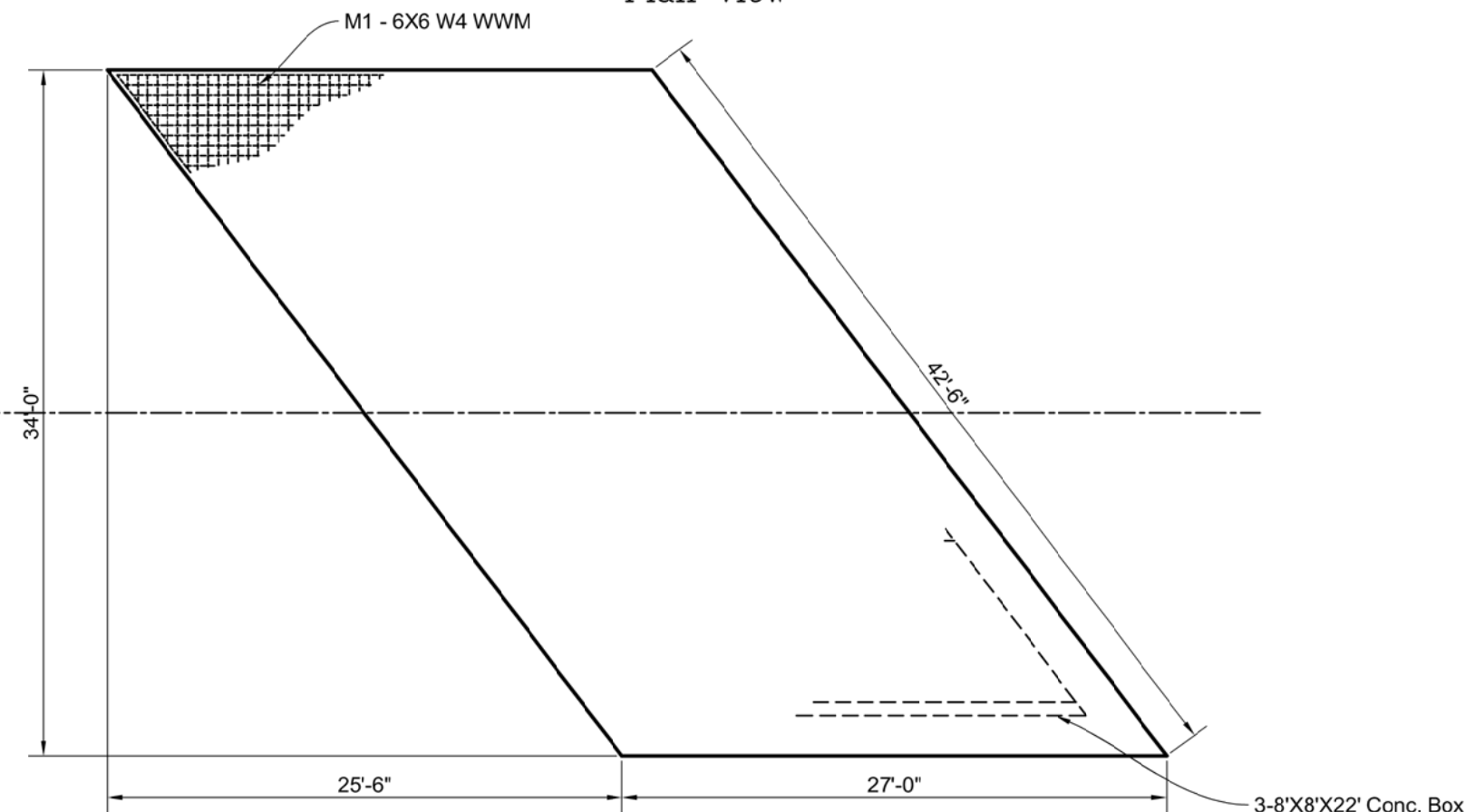
Seal Slab Detail (If Req'd)
