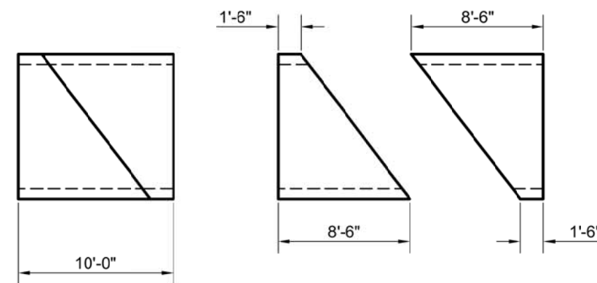
8'X8'X10' Special Box Detail
